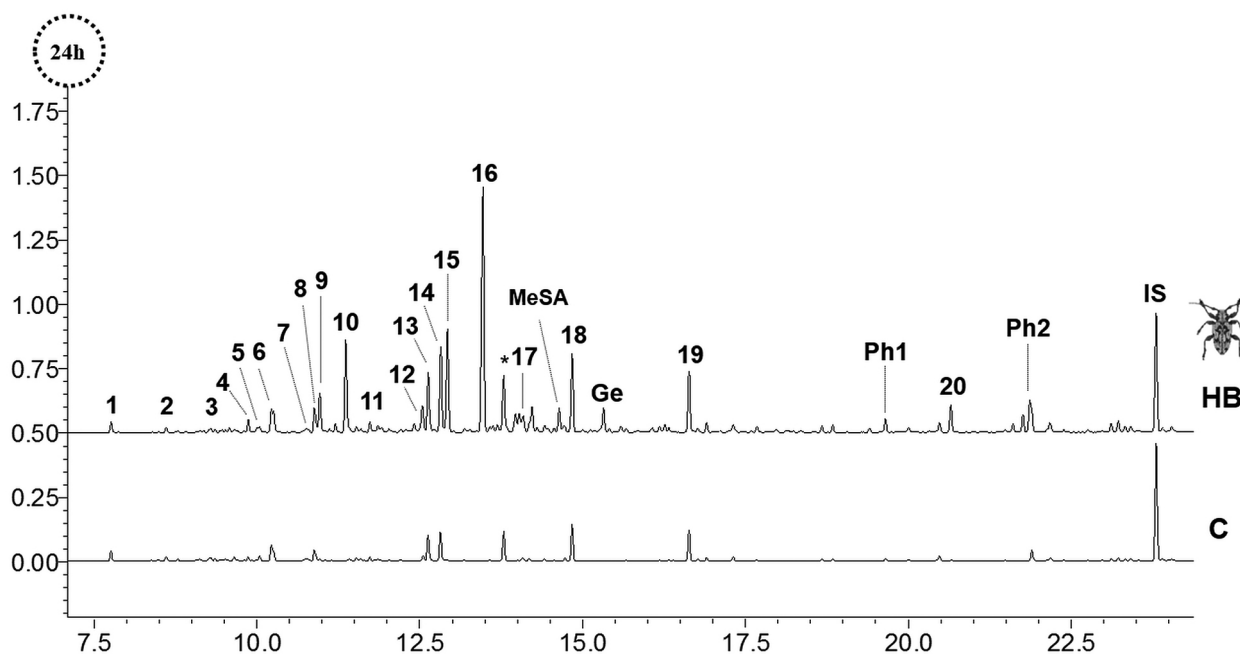
Figure 1. Comparisons of the chromatograms of Ilex paraguariensis extracts (24 h) treated with the herbivory of Hedypathes betulinus (HB) and control plants (C). HB chromatogram represents the VOCs (1–20) emitted by yerba mate plants. MeSA: methyl salicylate; Ge: geraniol; components of H. betulinus pheromone, Ph1 and Ph2: ( E )-6,10-dimethyl-5,9-undecadien-2-one (geranylacetone) and ( E )-6,10-dimethyl-5,9-undecadien-2-yl acetate, respectively.
