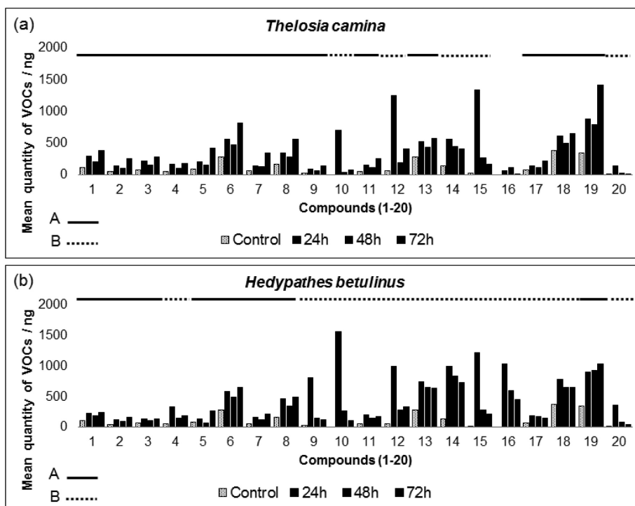
Figure 3. Graphical representation of the two different patterns of emissions (A: solid line and B: dotted line) of the VOCs (1-20) from Ilex paraguariensis control plants and herbivory treated plants: (a) Thelosia camina ; (b) Hedypathes betulinus , according to time (24-72 h). In pattern A: peak of emission at 72 h or up regulated; in pattern B: peak of emission at 24 h or down regulated.
