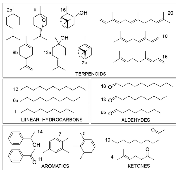
Figure 2. VOCs (1–20) emitted from Ilex paraguariensis plants treated with the herbivory by Thelosia camina (TC), Hedypathes betulinus (HB), mechanical damage (MD) and control. Compound names are in Table 1.
