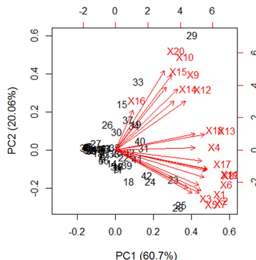
Figure 4. PCA plot representing VOCs 1-20 (X1 - X20) distributed on PC1 and PC2. VOCs emitted from Ilex paraguariensis plants treated with the herbivory by Thelosia camina (TC), Hedypathes betulinus (HB), mechanical damage (MD) and control.
