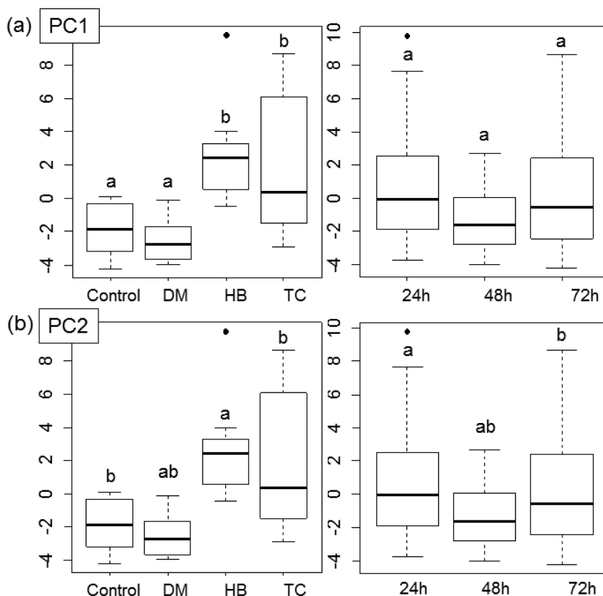
Figure 5. PCs 1 (a) and 2 (b): comparisons of treatments (control, mechanical damage (MD), and herbivories by Hedypathes betulinus (HB) and Thelosia camina (TC)) and times (24, 48, and 72 h). Different letters indicate significant differences.
