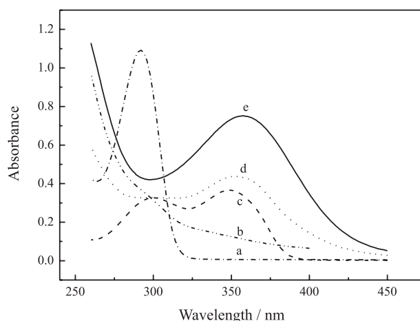
Figure 4. UV spectra of UA (a), UA-Ag(III) (b), Ag(III)-luminol (c), luminol (d), and Ag(III) (e). The concentrations of UA, luminol and [Ag(HIO 6 ) 2 ] 5- in mixed solution were all 5.0 \times 10^{-5} mol L -1 .
